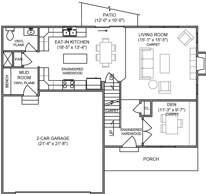
main floor
